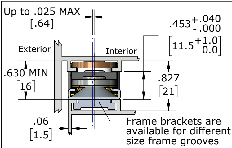
TYPE 1 Eurogroove with .025 offset 40B2001 EZi Hinge (Groove A)
