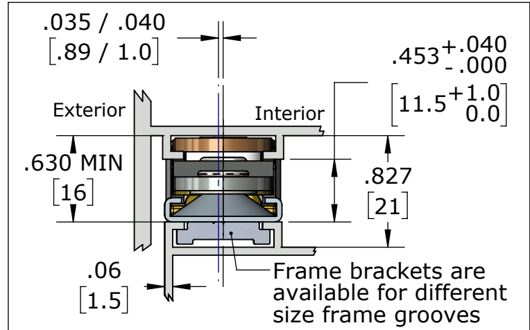
TYPE 1 Eurogroove with .040 offset 40B2003 EZi Hinge (Groove B)
