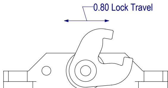
300-Series Stainless Steel Socket & Drive Arm. Diecast Housing.
