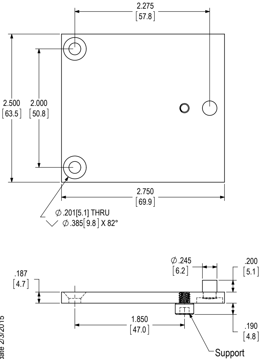
1625 Offset Drive Plate
