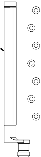
1.75" Bottom End Pivot Hinge Assy - RIGHT 41D0090002 (See Sheet 33)
