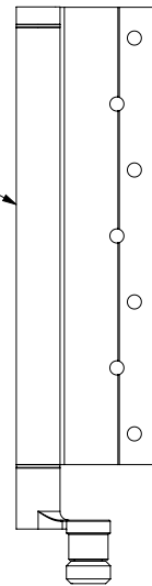
1.75" Bottom End Pivot Hinge Assy - Offset Left 41D0090001 (See Sheet 32)
