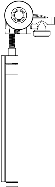
Series C - 2.00" End Hanger Assy - RIGHT 41D0214001 (See Sheet 60)
