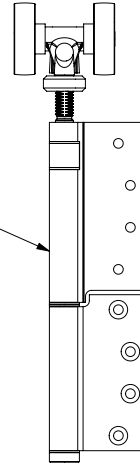
Series C - 1.75" Intermediate Hanger Assy 41D0215002 (See Sheet 63)
