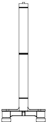
1.75" Bottom Intermediate Guide Assy 41D0155002 (See Sheet 49)
