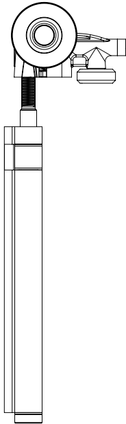
Series C - 1.75" End Hanger Assy - LEFT 41D0213002 (See Sheet 59)
