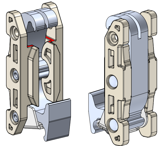
21B310 ECO Carrier Assembly
