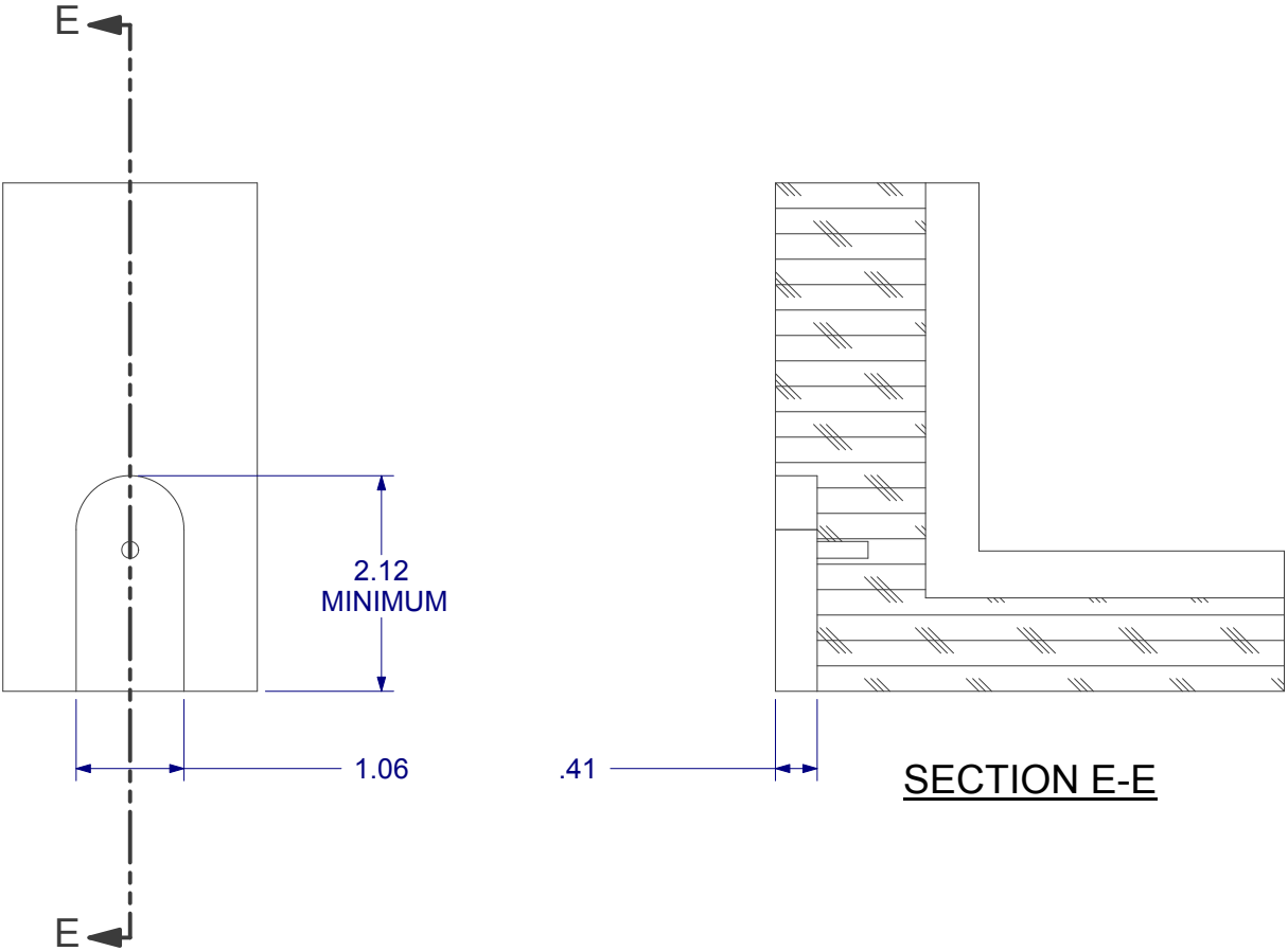
SASH CORNER CUT OUT
