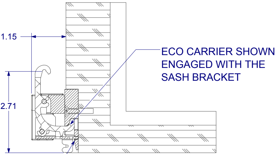
TAKE-OUT BRACKET SHOWN IN THE STORED POSITION CROSS SECTION
