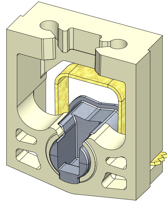
Carrier Assembly 15B100 (Locked Position)
