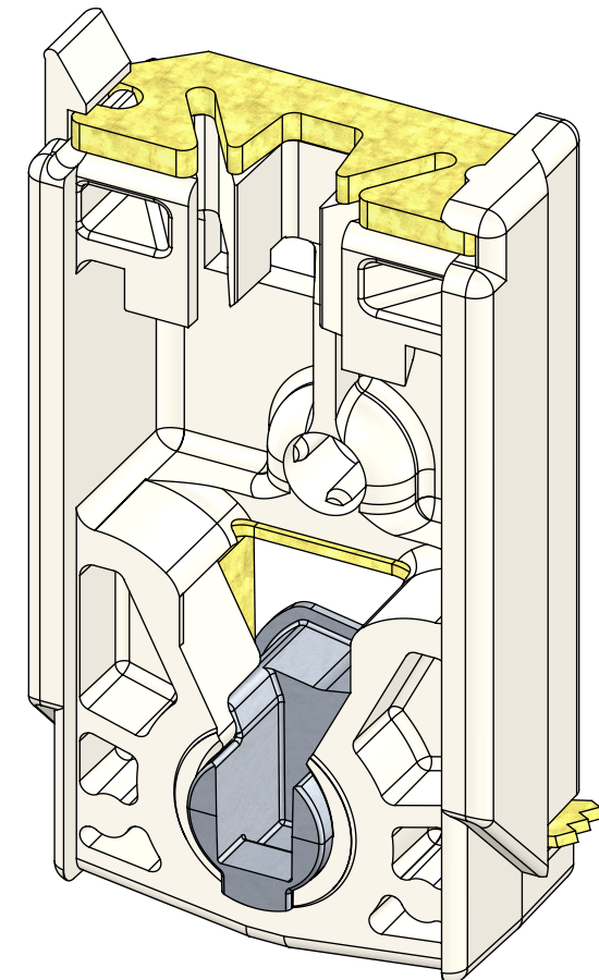
.625 Carrier Assembly 15B110 (Locked Position)
