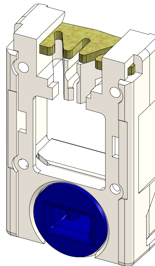
Carrier Assembly 16H65 (Unlocked Position)
