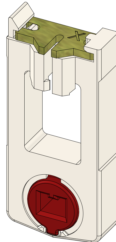
Carrier Assembly 16L05 (Unlocked Position)
