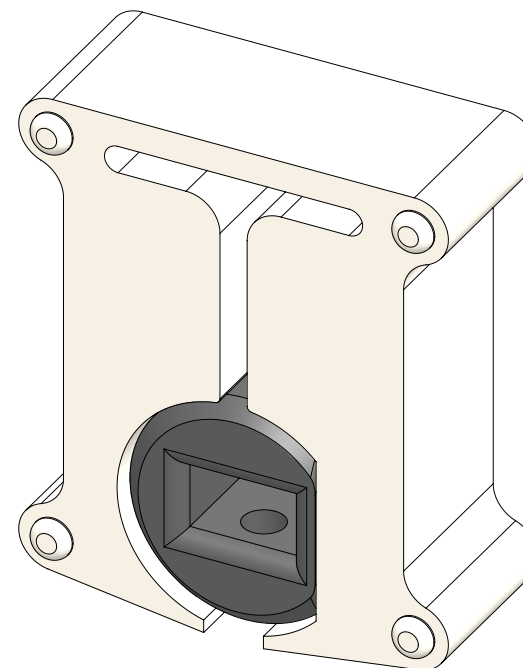
16T165 Slider Carrier Assembly
