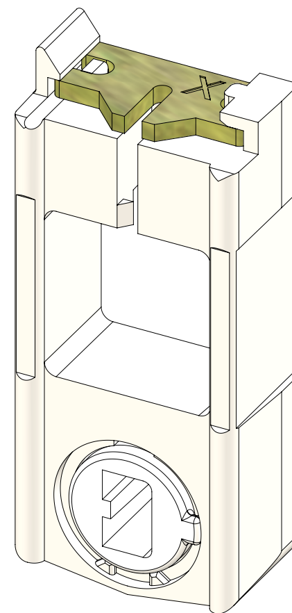
Carrier Assembly 16T225 (Unlocked Position)
