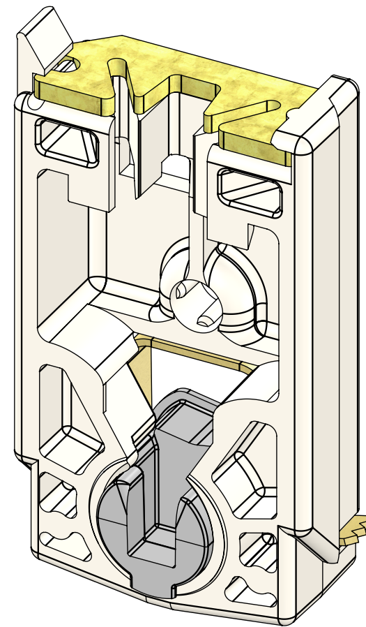
.562" Carrier Assembly (High Torque Positive Lock) 20B0010 (Locked Position)
